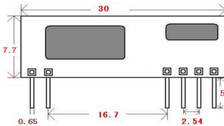
CY120 Dimension
