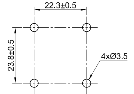
PCB/MOUNTING LAYOUT
