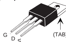
TO-220 (IXFP)
