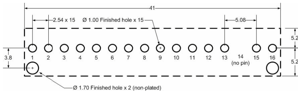
Figure 48. Recommended Footprint – Top View (all dimensions in mm)
