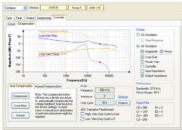
Figure 37. POL Controller Compensation Window
