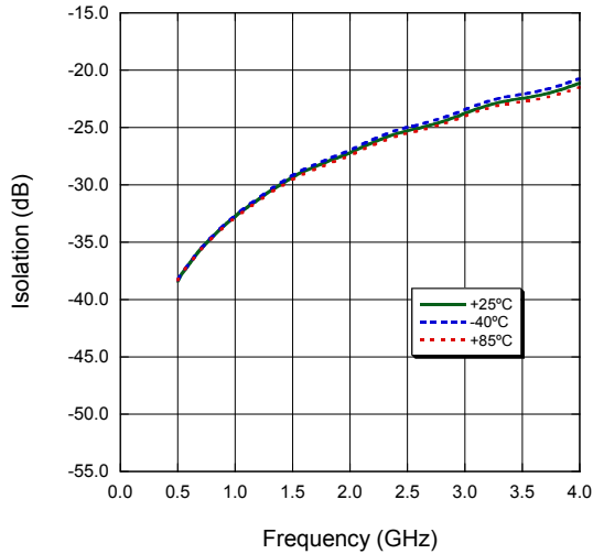
MASW-000825-12770T, TX Isolation Vs. Temperature Bias: +28V @ 0mA
