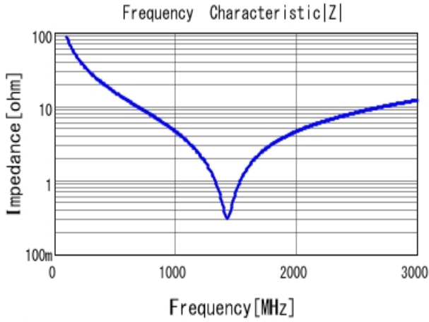
■ GRM21A5C2E180JW01 |Z| DCOV, 25degC
