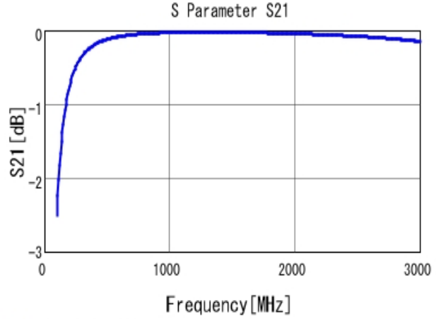
■ GRM21A5C2E180JW01 S21 DCOV, 25degC
