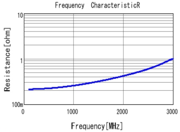
■ GRM21A5C2E180JW01 R DCOV, 25degC
