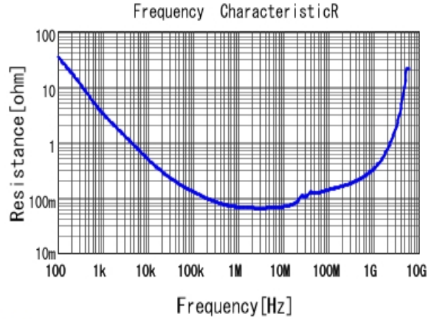
■ GCJ31MR72A224KA01 R DCOV, 25degC
