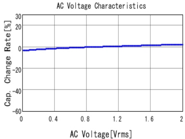
■ GCJ31MR72A224KA01 C-AC Voltage capchange, DCOV, 25.0d
