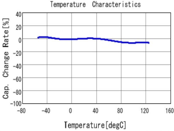
■ GCJ31MR72A224KA01 C-Temp. capchange, DC0.0V, AC1.0V r m
