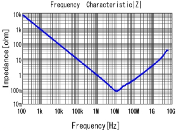
■ GCJ31MR72A224KA01 |Z| DCOV, 25degC
