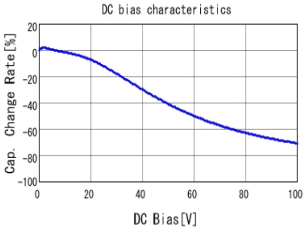
■ GCJ31MR72A224KA01 C-DC bias capchange, 25.0degC, AC1.
