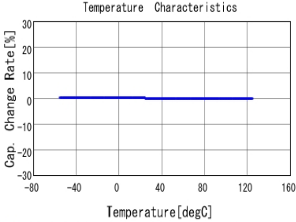
■ GRM1555C1H390GA01 C-Temp. capchange, DCOV, AC1Vrms
