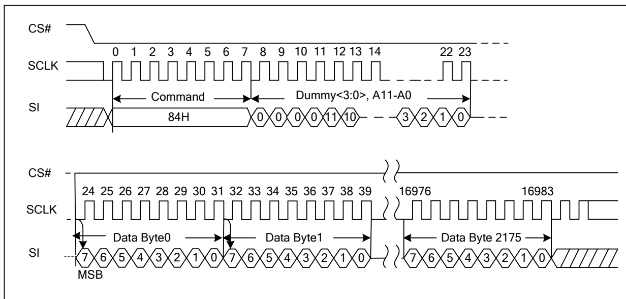
Figure19. Program Load Random Data Sequence Diagram
