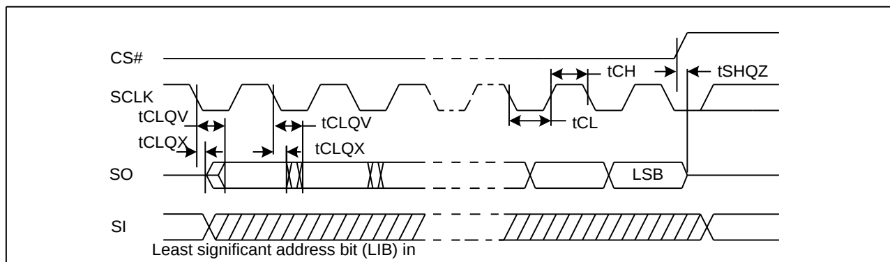
Figure26. Output Timing
