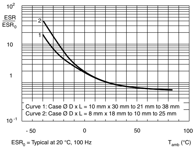
Fig. 6 - Typical multiplier of ESR as a function of ambient temperature
