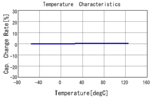
GRM31A5C2J101JW01 C-Temp. capchange, DCOV, AC1Vrms
