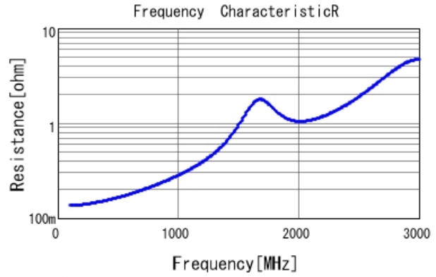
GRM31A5C2J101JW01 R DCOV, 25degC
