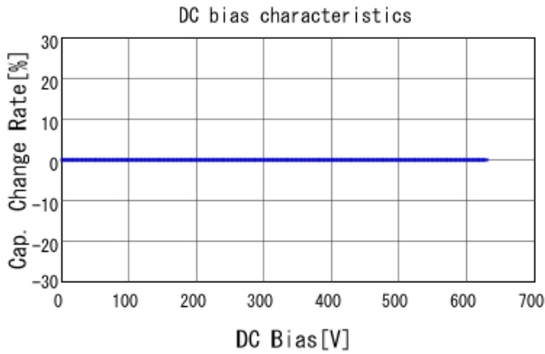
GRM31A5C2J101JW01 C-DC bias capchange, 25.0degC, A
