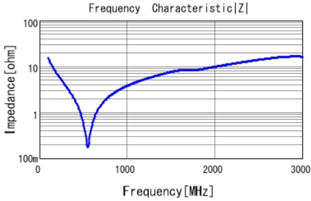
GRM31A5C2J101JW01 |Z| DCOV, 25degC
