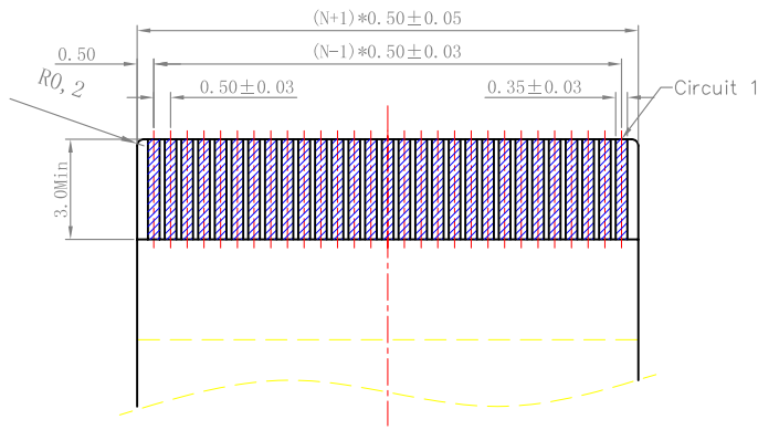
RECOMMENDED FPC/FFC DIMENSION
