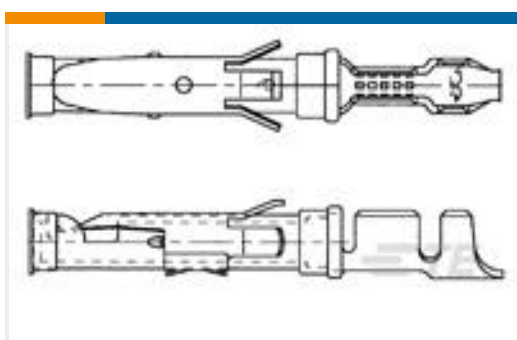
TE Part #163088-1 062 SOC.ASS. TYP3+
