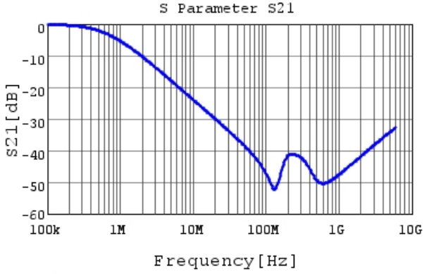
NFM31KC103R1H3 S21 DCOV,25degC, Feedthrough
