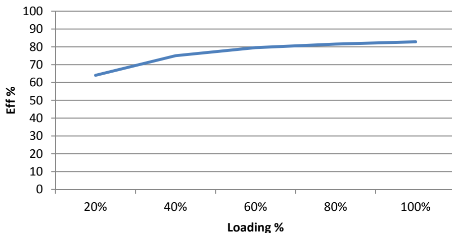
AM3T-2412S-VZ Efficiency vs. Loading
