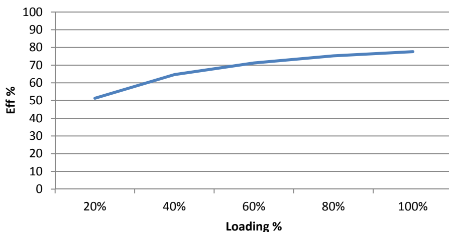
AM3T-4815S-VZ Efficiency vs. Loading
