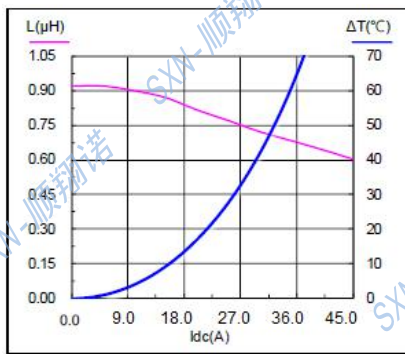
SMMS1050-R82M
