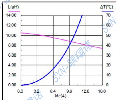
SMMS1350-100M
