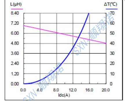
SMMS1360-6R8M
