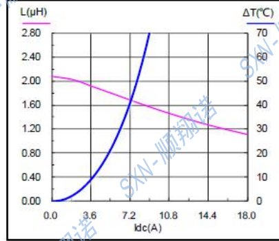
SMMS0624-2R2M
