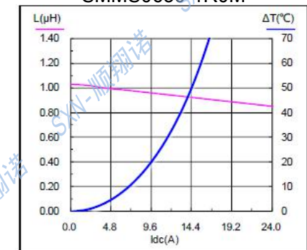
SMMS0630-1R0M
