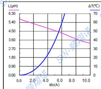
SMMS0624-100M
