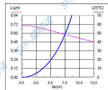
SMMS0420-R68M
