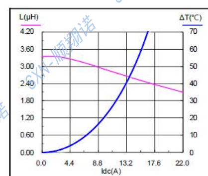
SMMS1050-3R3M
