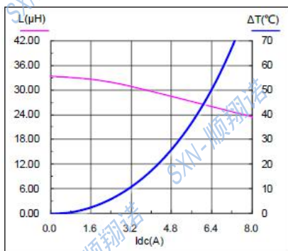
SMMS1350-330M
