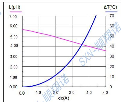
SMMS0520-5R6M
