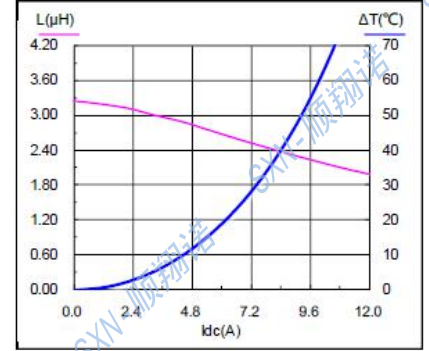
SMMS0650-3R3M
