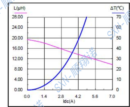
SMMS0650-680M
