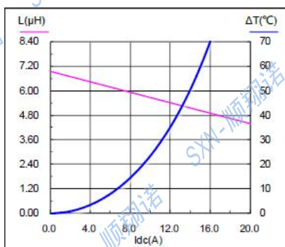
SMMS1350-6R8M
