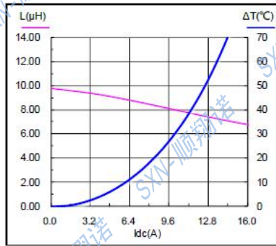
SMMS1360-100M
