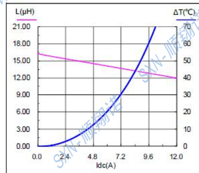
SMMS1350-150M
