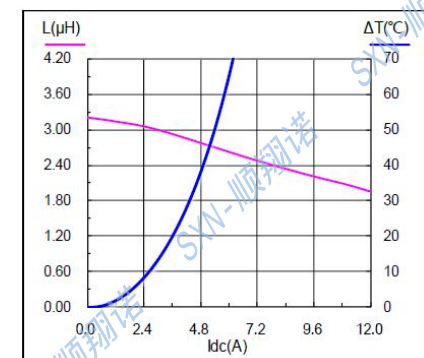
SMMS0530-100M
