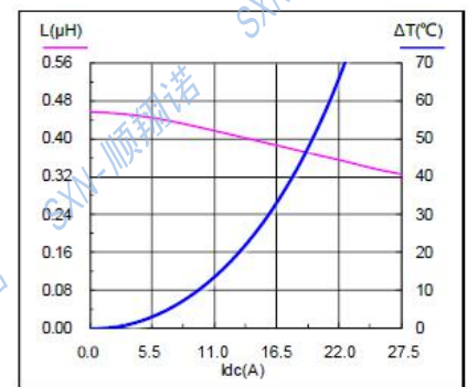
SMMS0624-R47M
