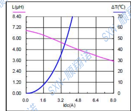
SMMS0624-6R8M
