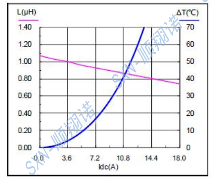
SMMS0624-3R3M
