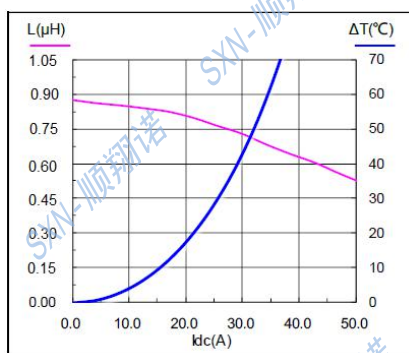
SMMS1350-R82M
