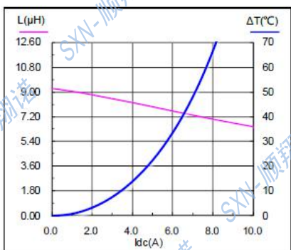
SMMS1040-330M
