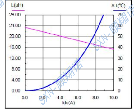
SMMS1360-220M
