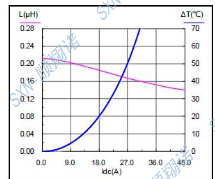
SMMS0630-R22M
