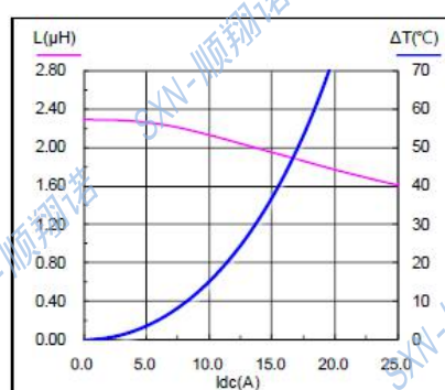
SMMS1050-2R2M
