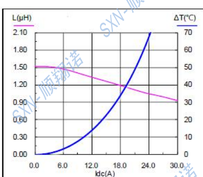
SMMS1050-1R5M
