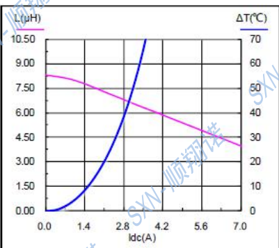
SMMS0624-8R2M
