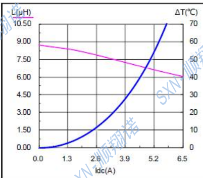
SMMS0630-8R2M
