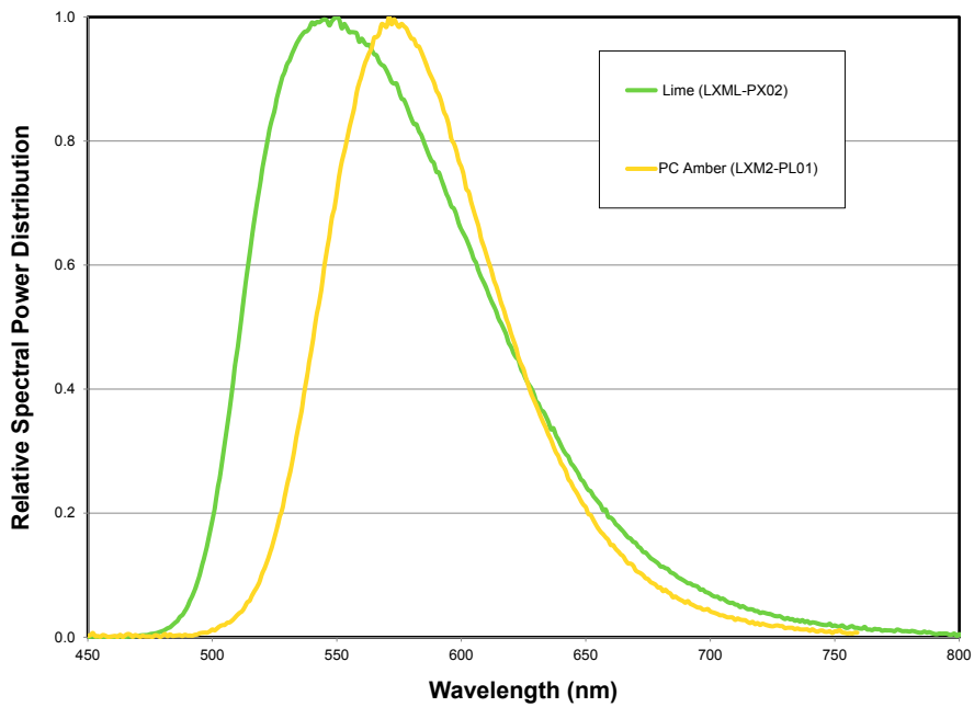
Figure 1b. Typical normalized power vs. wavelength for LUXEON Rebel PC Amber and Lime at 350mA, test temperature.
