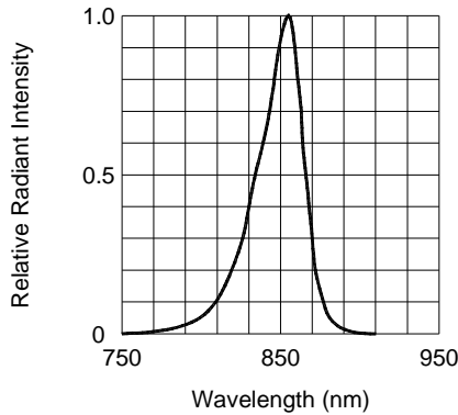
FIG.1 SPECTRAL DISTRIBUTION 15A047 20mA
