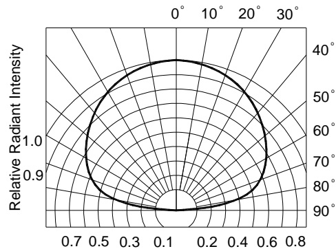
FIG.6 RADIATION DIAGRAM
