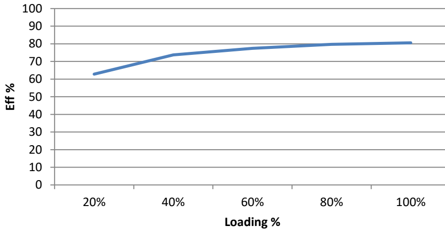
AM3G-2412SZ Efficiency vs. Loading
