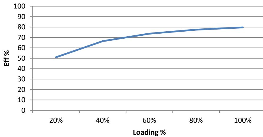
AM2GH-1205Z Efficiency vs. Loading
