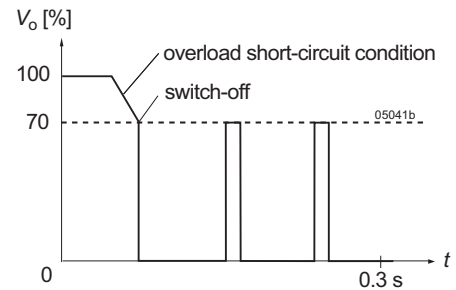
Fig. 6 Overload switch off (hiccup mode), typical values.
