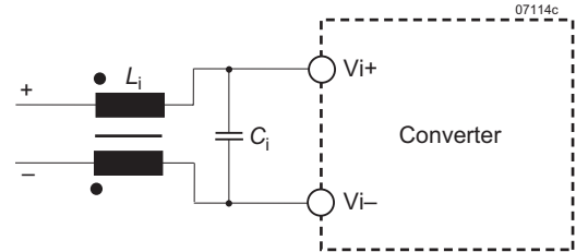
Fig. 15 External filter circuitry
