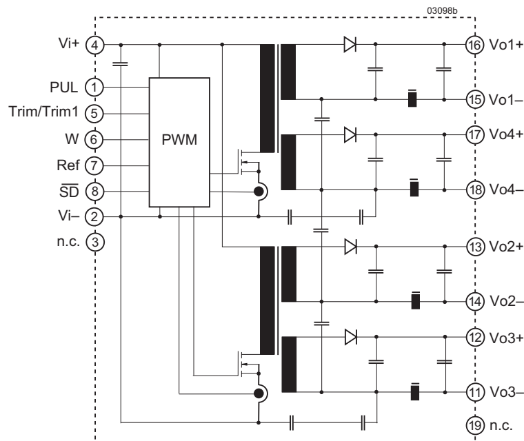
Fig. 1 Block diagram of quad-output models
