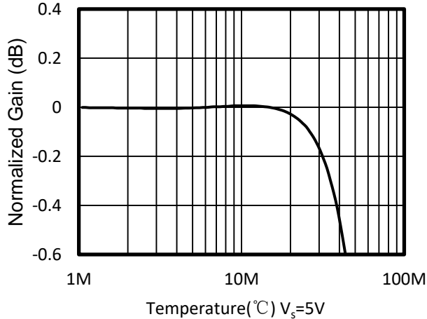
AC Response
