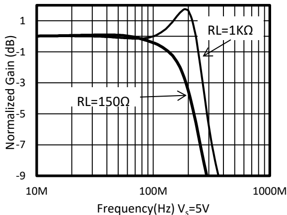
-3dB_GW_Gain=1
