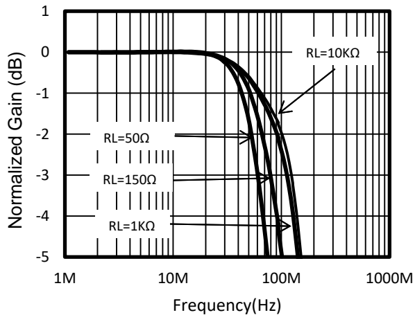
-3dB_GW_Gain=2
