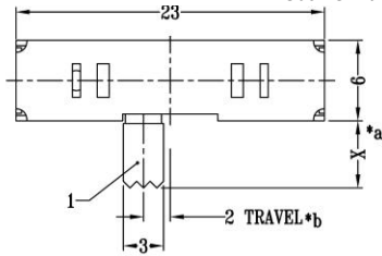
Outline Drawing
