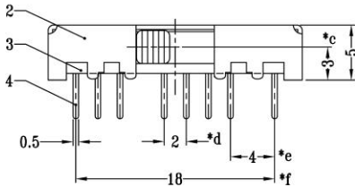
Mounting
