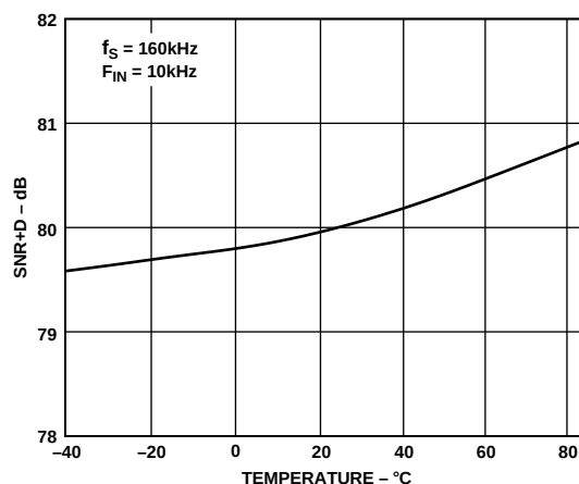
Figure 14. SNR + D vs. Temperature
