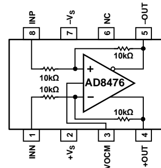
Figure 1. 8-Lead MSOP
