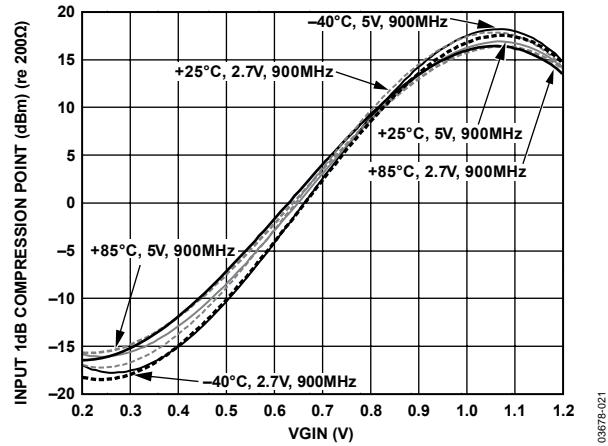
Figure 21. Input 1 dB Compression Point ( IP1dB ) vs. V_{GIN} , F_{IF} = 900\text{ MHz} , F_{BB} = 1\text{ MHz} , V_{POS} = 2.7\text{ V} , 5\text{ V} , Temperature = -40^\circ\text{C} , +25^\circ\text{C} , +85^\circ\text{C}
