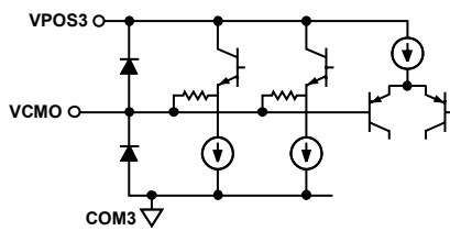
Figure 5. Circuit C
