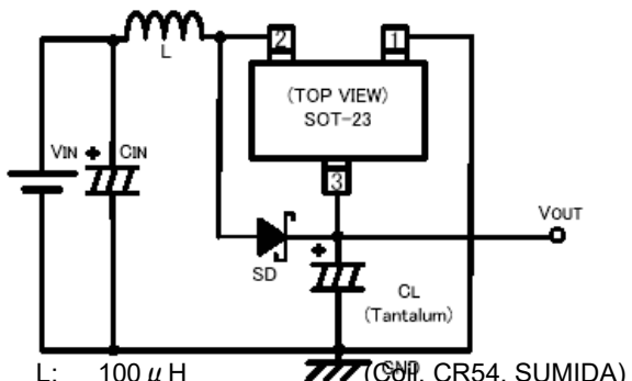
●A type circuit
