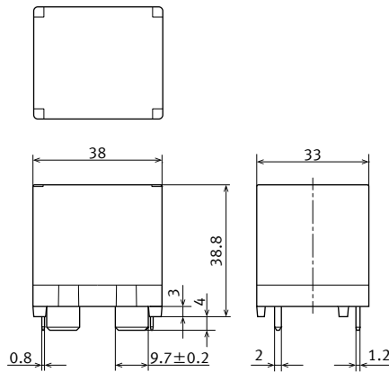
External dimensions
