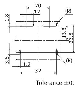
Recommended PC board pattern (BOTTOM VIEW)
