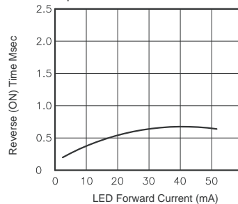
Fig.11 LED forward current vs. reverse time Across terminals 7 and 8 pin; Load voltage: 400V (DC); Continuous load current: 130mA (DC); Ambient temperature: 25°C
