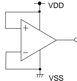
Figure 27. Example of Application Circuit for Unused Comparator
