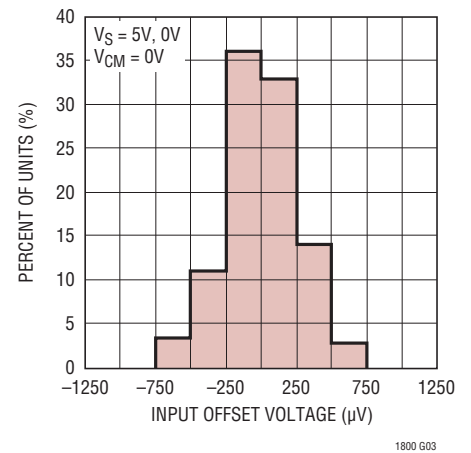
V_{OS} Distribution, V_{CM} = 0\text{V} (SOT-23, PNP Stage)
