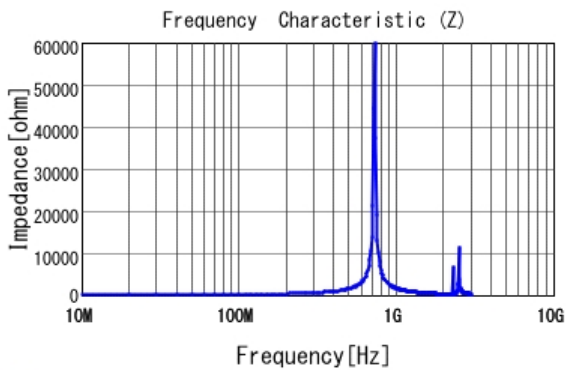
■ LQW2UASR27J00 |Z|
