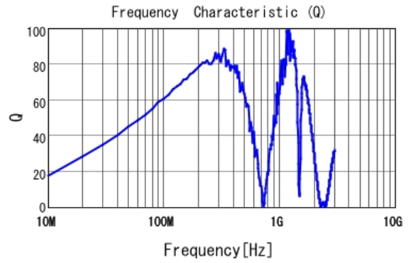
■ LQW2UASR27J00 Q
