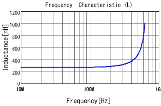
■ LQW2UASR27J00 L
