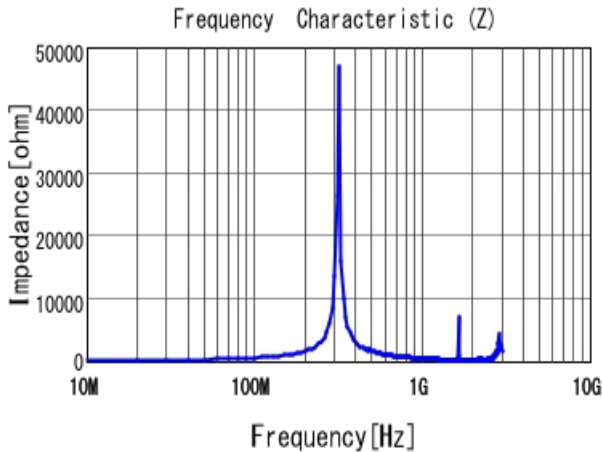
■ LQW2BASR82J00 |Z|
