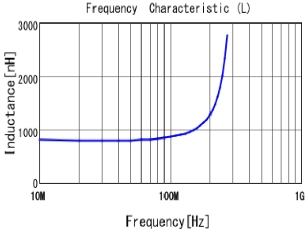
■ LQW2BASR82J00 L
