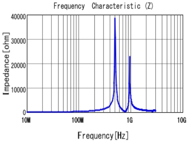
■ LQW2BASR47J00 |Z|
