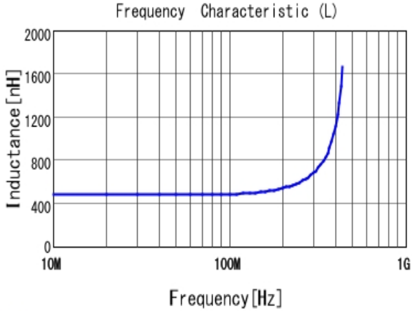
■ LQW2BASR47J00 L
