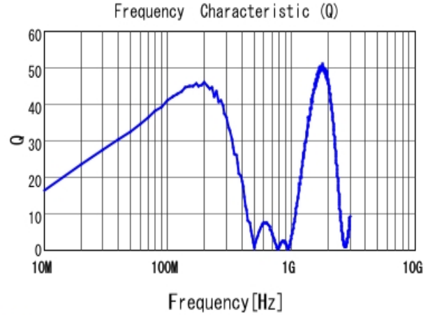
■ LQW2BASR47J00 Q
