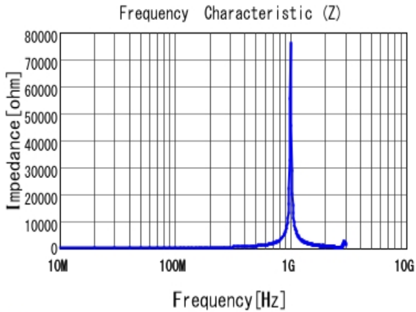
■ LQW2BASR22J00 |Z|
