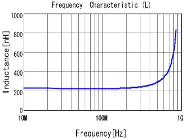
■ LQW2BASR22J00 L
