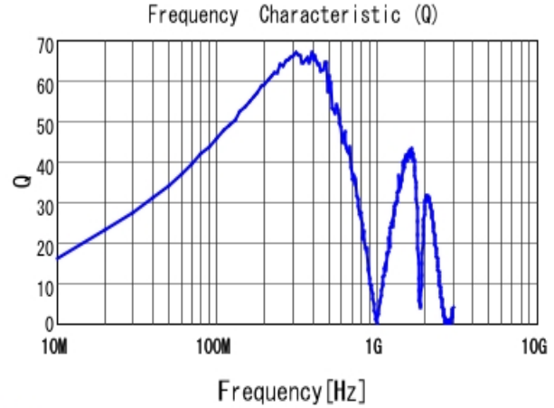
■ LQW2BASR22J00 Q
