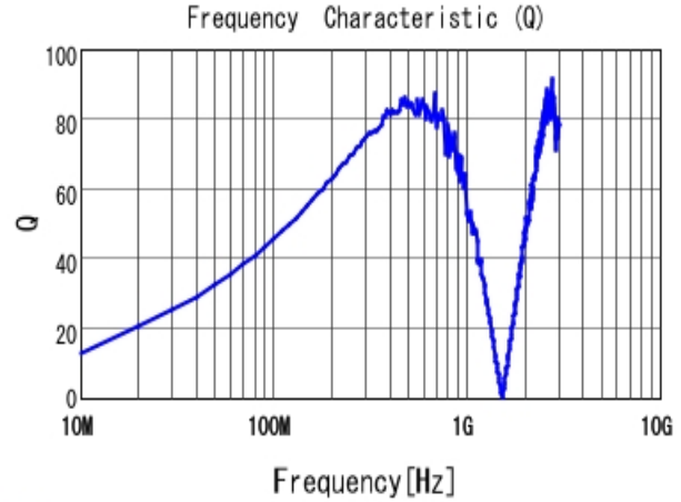
■ LQW2BASR10G00 Q
