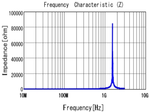
■ LQW2BASR10G00 |Z|
