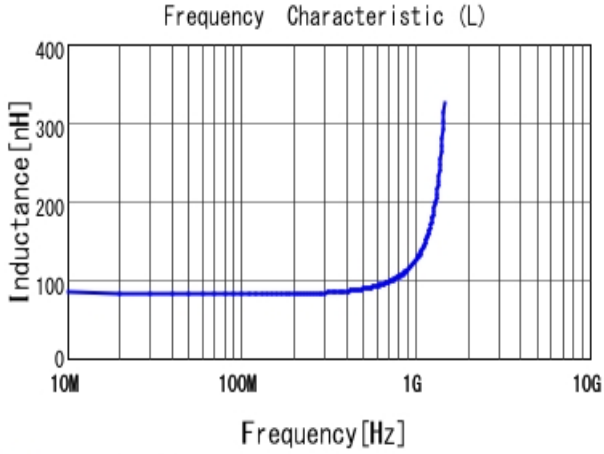
■ LQW2BAS82NJ00 L
