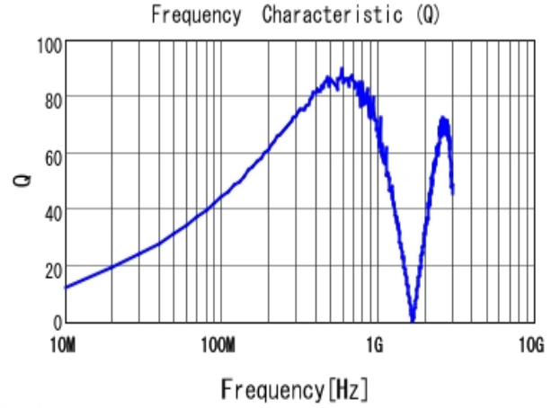
■ LQW2BAS82NJ00 Q
