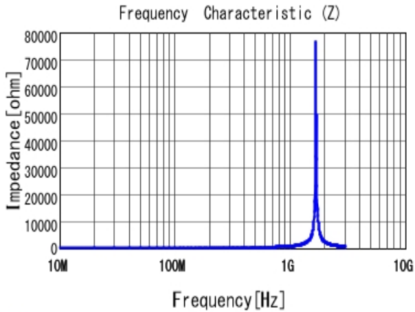
■ LQW2BAS82NJ00 |Z|
