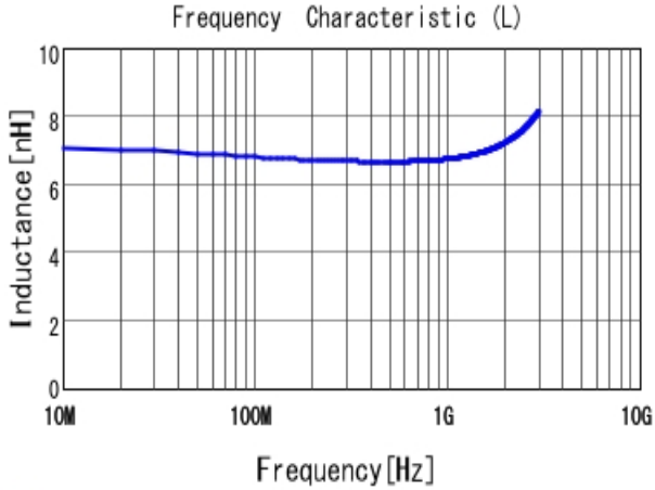
■ LQW2BAS6N8J00 L
