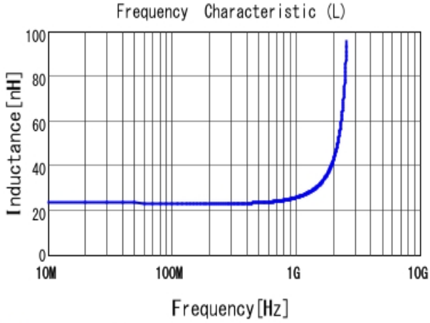
■ LQW2BAS24NJ00 L
