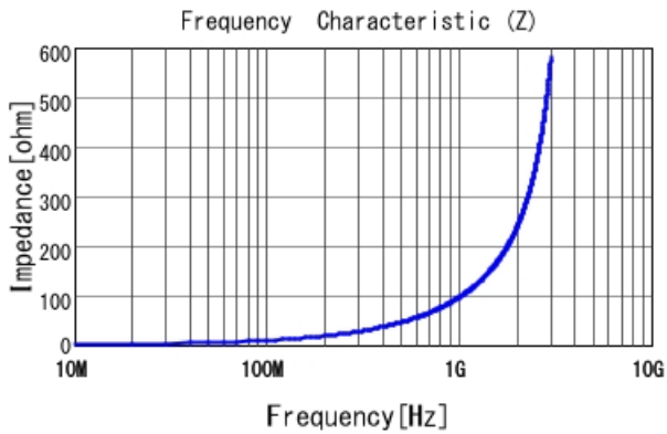
■ LQW2BAS15NJ00 |Z|
