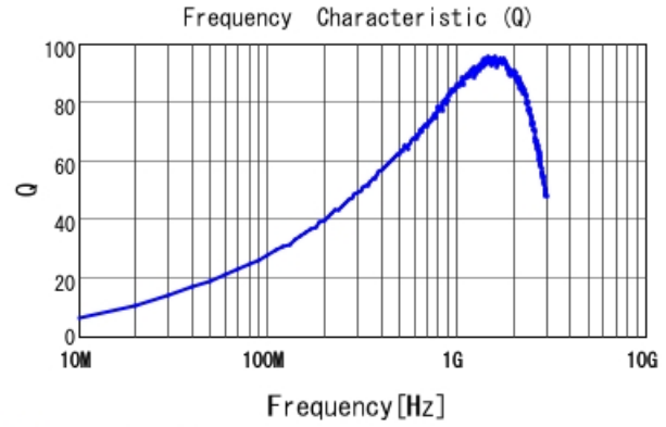
■ LQW2BAS15NJ00 Q
