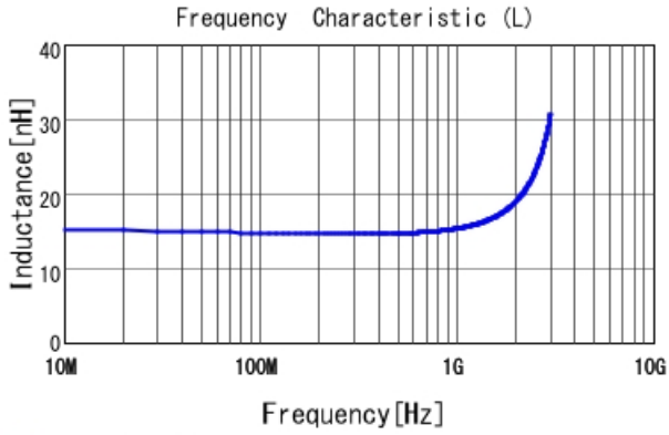
■ LQW2BAS15NJ00 L
