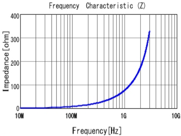
■ LQW2BAS12NJ00 |Z|
