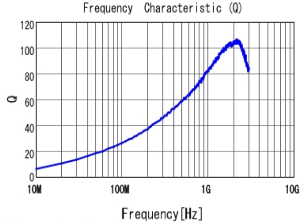
■ LQW2BAS12NJ00 Q
