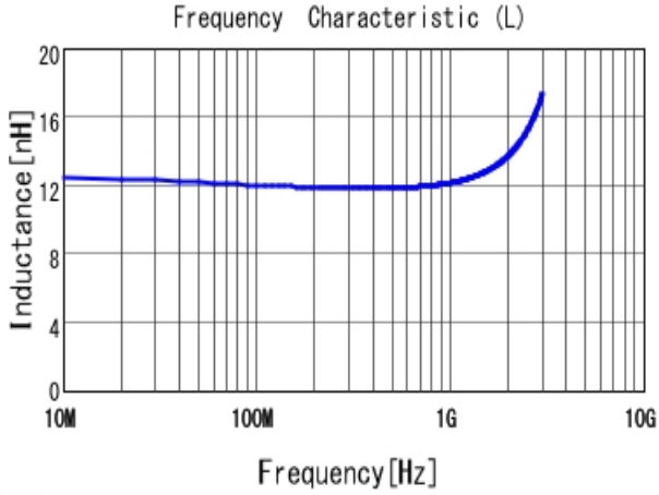
■ LQW2BAS12NJ00 L
