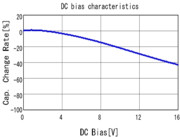
■ GRM32DR61C106KA01 C-DC bias capchange, 25.0degC, AC1.
