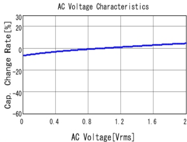
■ GRM32DR61C106KA01 C-AC Voltage capchange, DCOV, 25.0d
