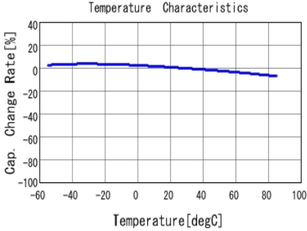
■ GRM32DR61C106KA01 C-Temp. capchange, DC0.0V, AC1.0V r m
