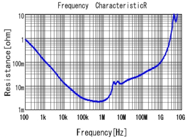
■ GRM32DR61C106KA01 R DCOV, 25degC
