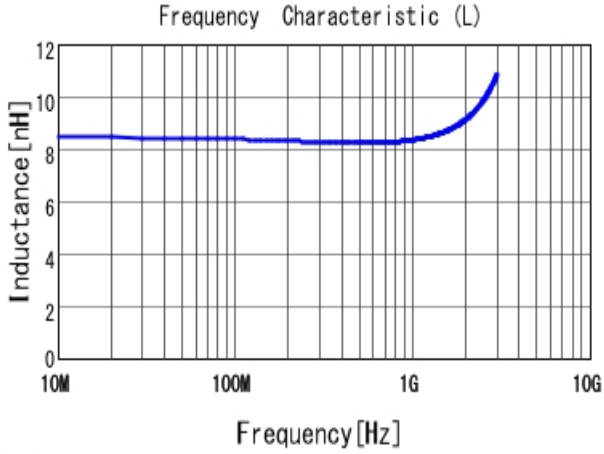
■ LQP15MN8N2B02 L
