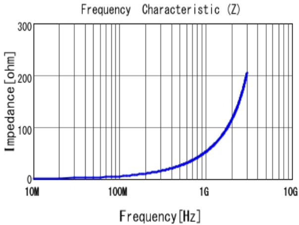
■ LQP15MN8N2B02 |Z|
