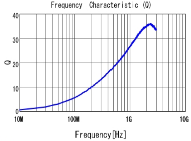
■ LQP15MN8N2B02 Q
