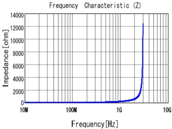
■ LQP15MN27NG02 |Z|
