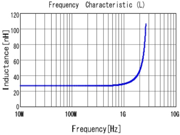
■ LQP15MN27NG02 L
