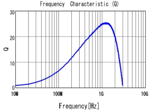
■ LQP15MN27NG02 Q
