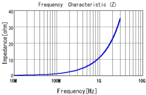
■ LQP15MN1N8W02 |Z|
