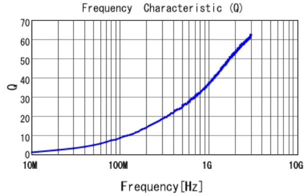
■ LQP15MN1N8W02 Q
