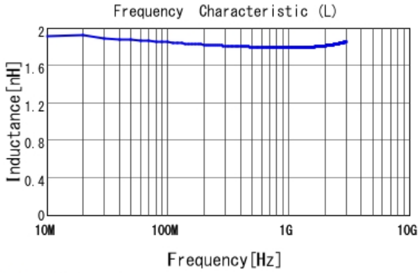
■ LQP15MN1N8W02 L
