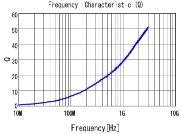
■ LQP15MN1N6B02 Q
