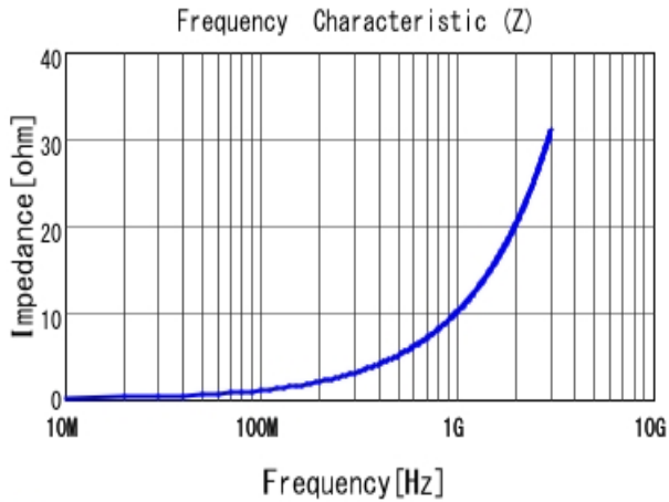
■ LQP15MN1N6B02 |Z|
