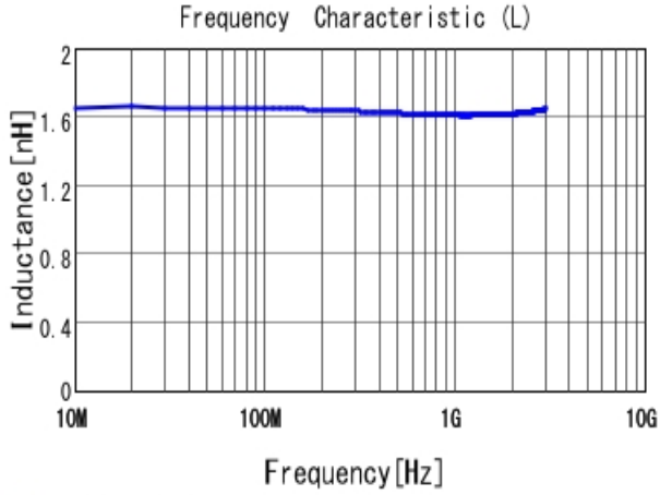
■ LQP15MN1N6B02 L
