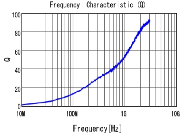
■ LQP15MN1N3B02 Q
