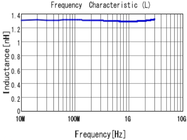
■ LQP15MN1N3B02 L
