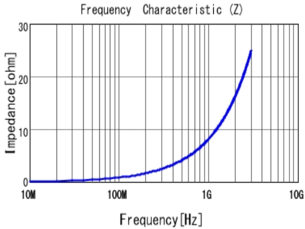
■ LQP15MN1N3B02 |Z|
