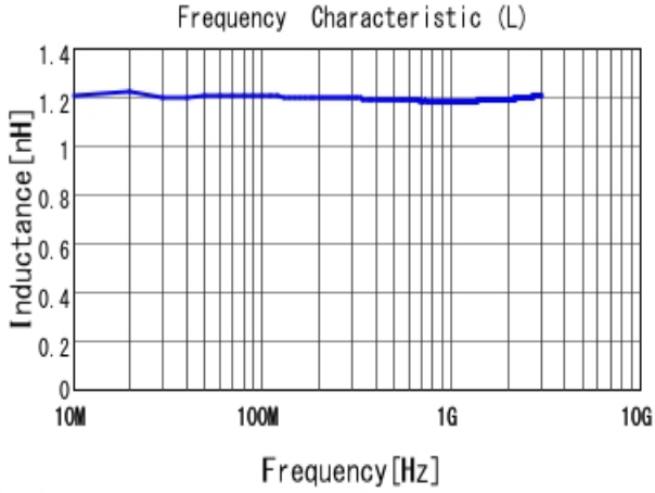
■ LQP15MN1N2B02 L
