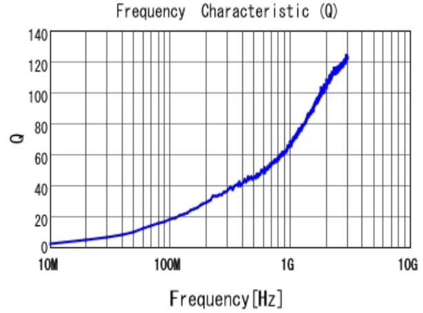
■ LQP15MN1N2B02 Q
