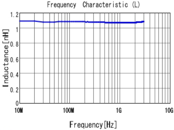
■ LQP15MN1N1W02 L
