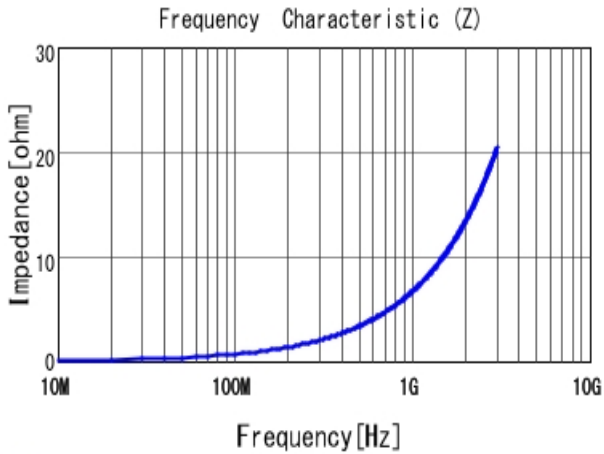
■ LQP15MN1N1W02 |Z|
