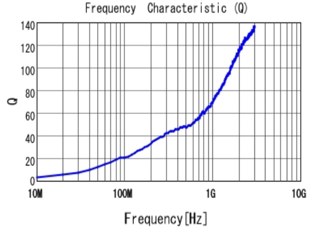
■ LQP15MN1N1W02 Q
